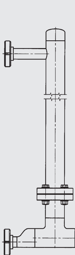
21 2 process connections per DIN 11851 Lower process connection via eccentric reducer
